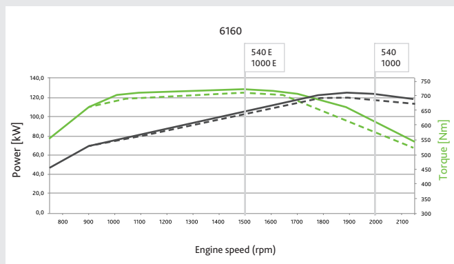
High performance engine curve of 6160.
