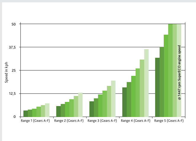
RCshift speeds: exceptional overlap of the different ranges and 50 kph superECO for maximum fuel efficiency (engine rpm with maximum tires size).
